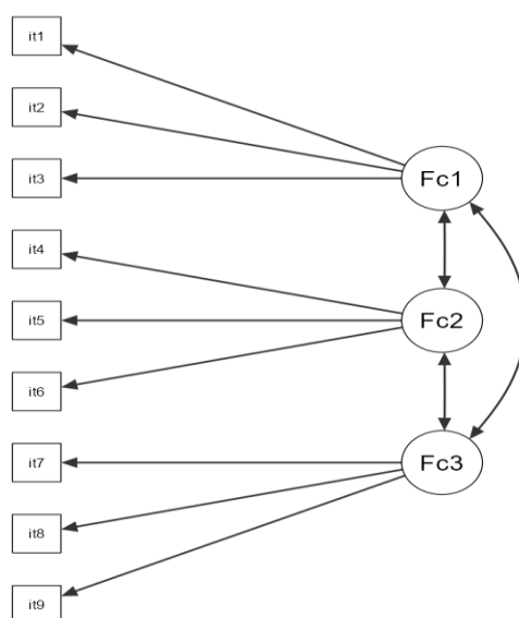
Figure 1. Path Diagram CFA
