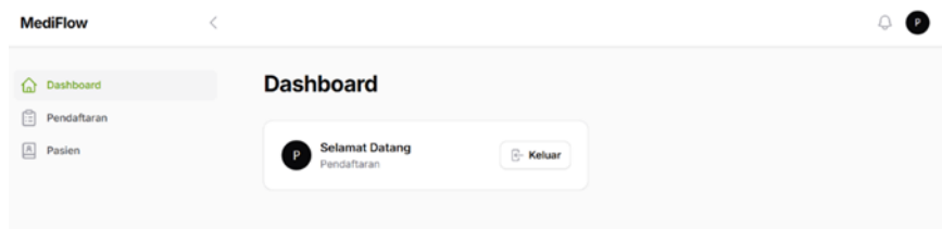
Figure 8. Dashboard
