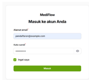
Figure 7. Login Page
