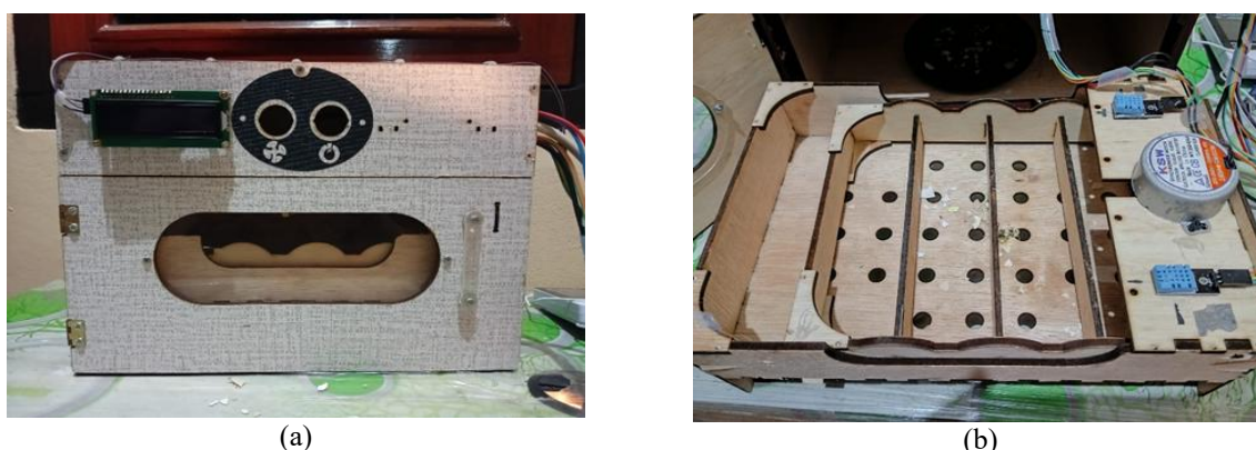
Figure 4. Prototype of egg hatcher front view and Top view of egg rack
