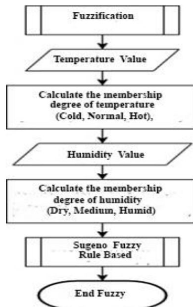
Figure 6. Fuzzification flowchart
